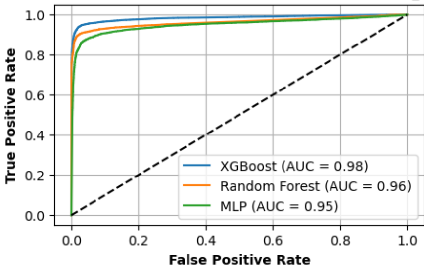
Receiver Operating Characteristic (ROC) Curve - Home-C_real
