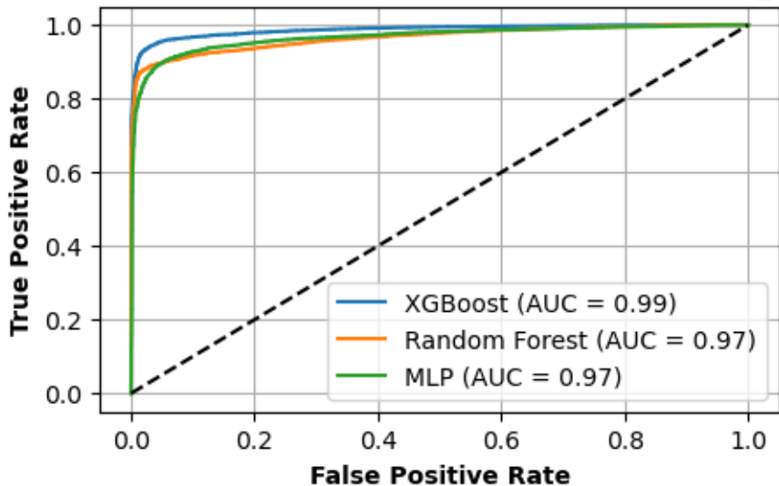
Receiver Operating Characteristic (ROC) Curve - Home-A_sim
