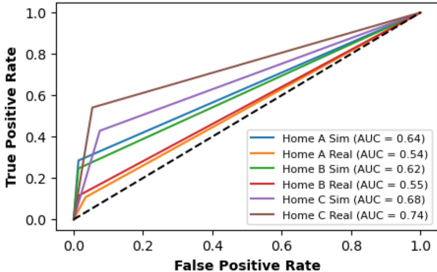
ROC Curve for Isolation Forest
