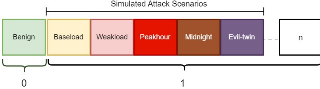
Figure 5.6: Multi-class attack scenarios with unspecified attacks preprocessed to binary attack class for anomaly detection.
