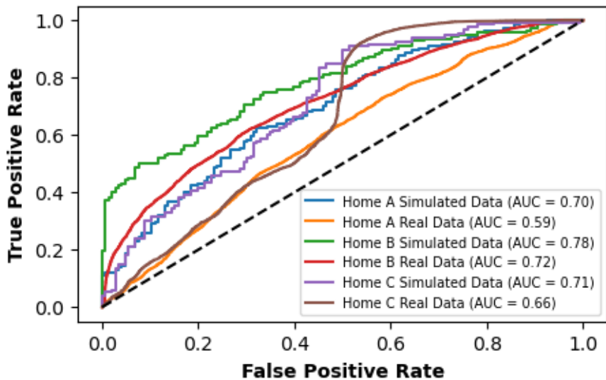
ROC Curve for LUM-1D-CONV-AE
