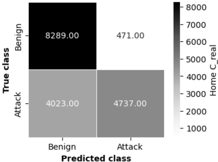
Confusion Matrix - IF Home C_real
