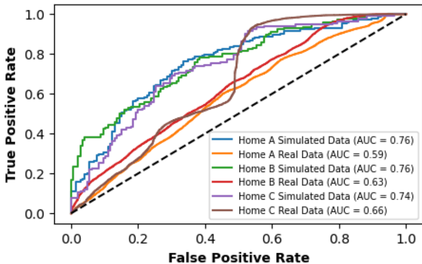
ROC Curve for LUM-MLP-AE
