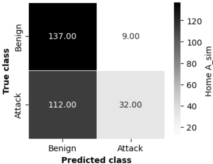
Confusion Matrix - MLP-AE Home A_sim
