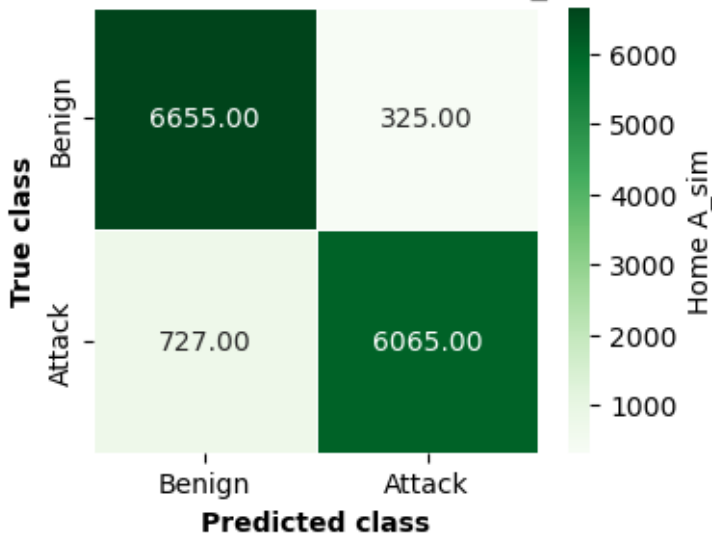
Confusion Matrix - MLP-Home A_sim
