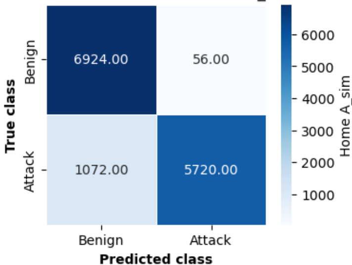
Confusion Matrix - RF-Home A_sim
