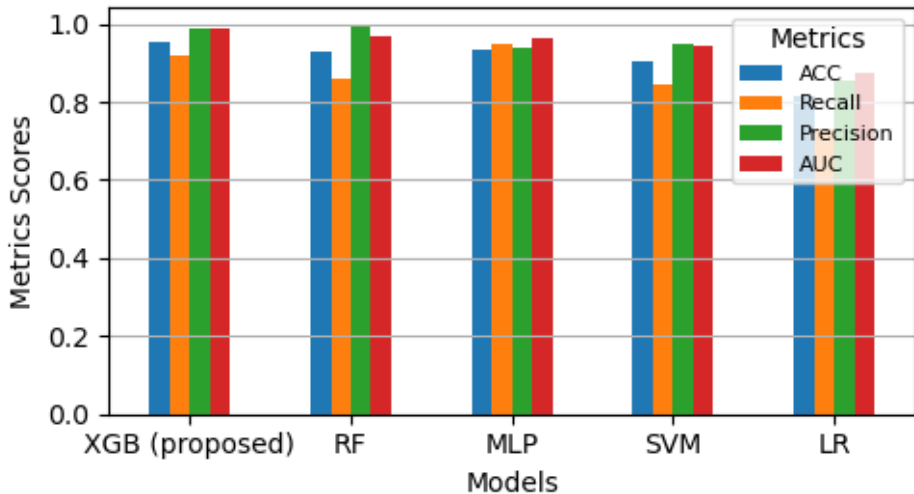
Performance metrics of binary classification models
