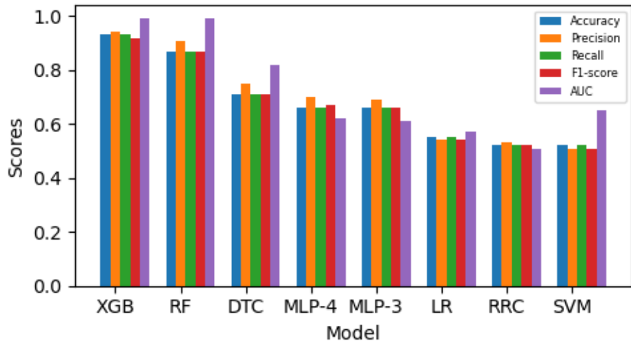
Performance Metrics of Different Multiclass Classification Algorithms
