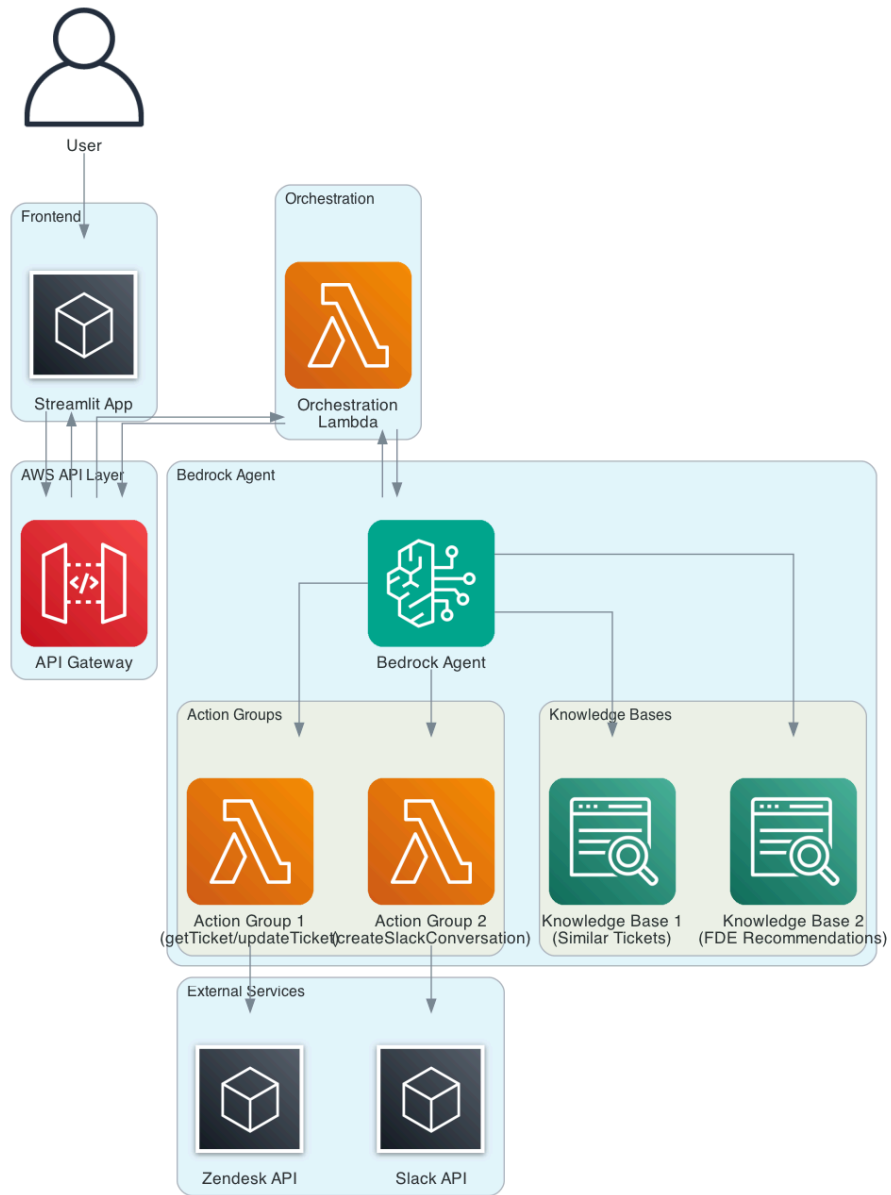
Streamlit-Bedrock-Zendesk Workflow
