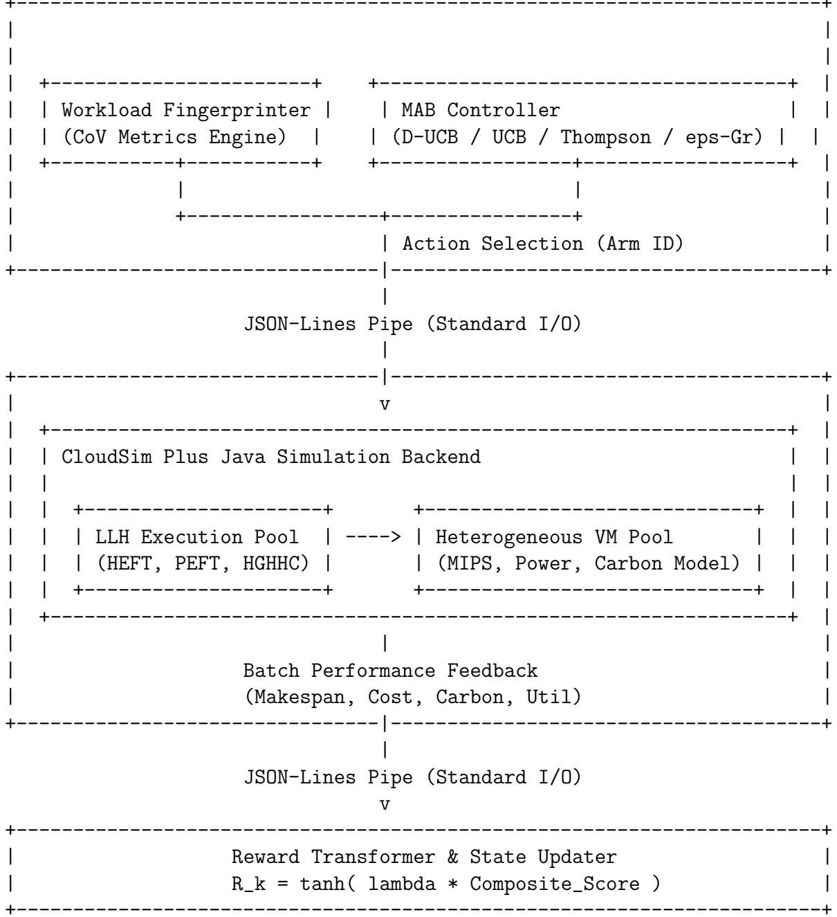
Figure 1: System Architecture showing the Python Hyper-Heuristic Engine linked via Standard I/O streaming pipes to the CloudSim Plus backend.
