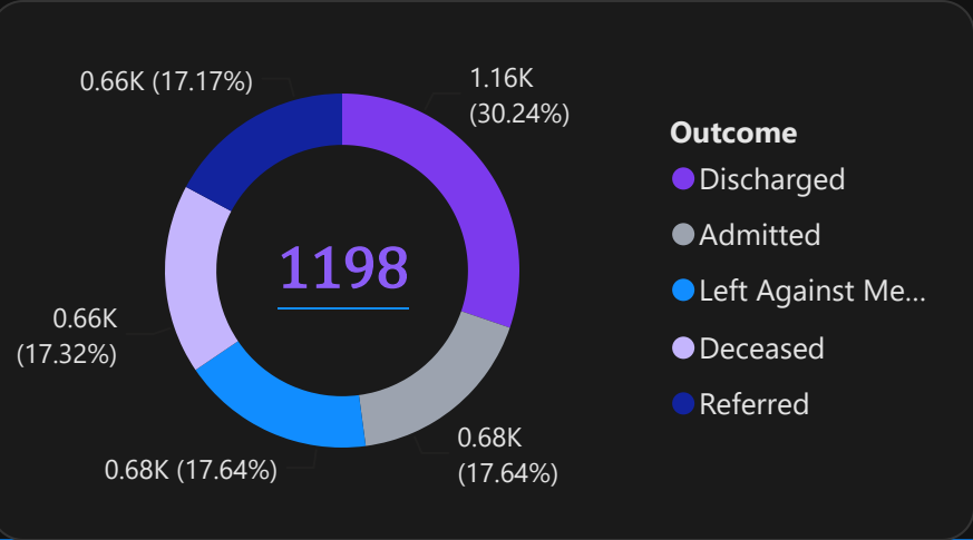
Patient Outcome
