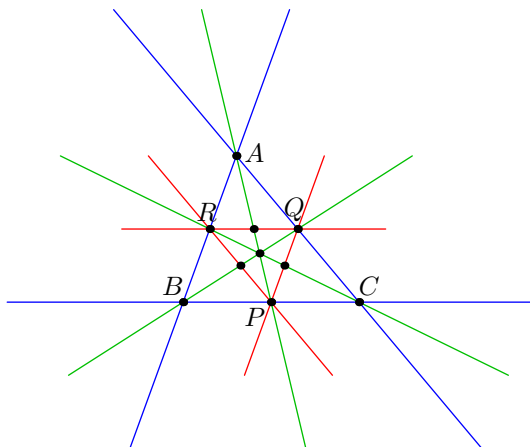
Figure 5: RMO 2025a P1, Exercise 1.5(b)(ii): Configuration with 9 lines and 10 intersection points.
