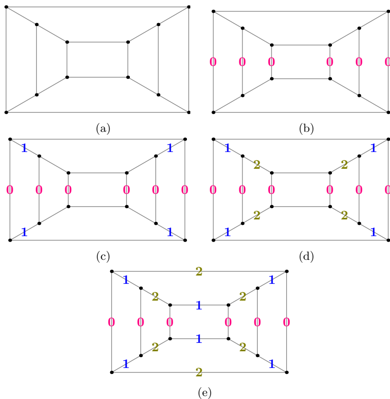
Figure 11: India RMO 2014, Example 1.17
