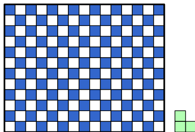
Figure 8: Tiling a 12 \times 15 chessboard using trominos.
