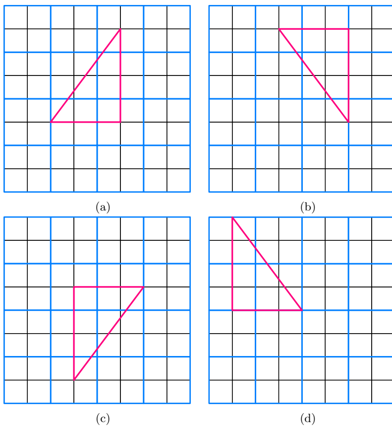
Figure 12: India RMO 2017b P1 — Several configurations of triangles with side lengths (3, 4, 5) , Example 1.22
