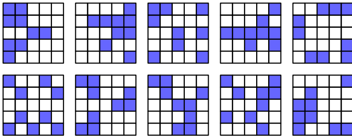
Figure 16: USAMO 2000 P4, Exercise 1.26
