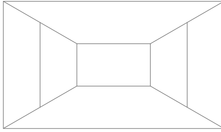
Figure 10: India RMO 2014d P6, Example 1.17
