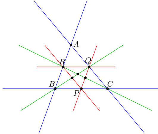
Figure 4: RMO 2025a P1, Exercise 1.5(b)(i): Configuration with 8 lines and 9 intersection points.
