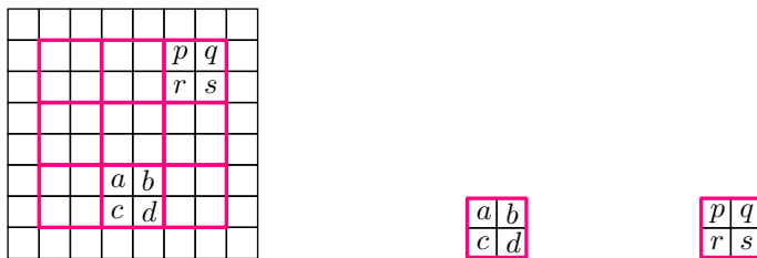
Figure 13: ad - bc = \pm 1, ps - qr = \pm 1 , Example 1.24
