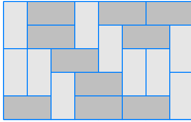
Figure 9: India BMath 2006 (a tiling of a 5 \times 8 rectangle with non-overlapping dominoes), Example 1.11
