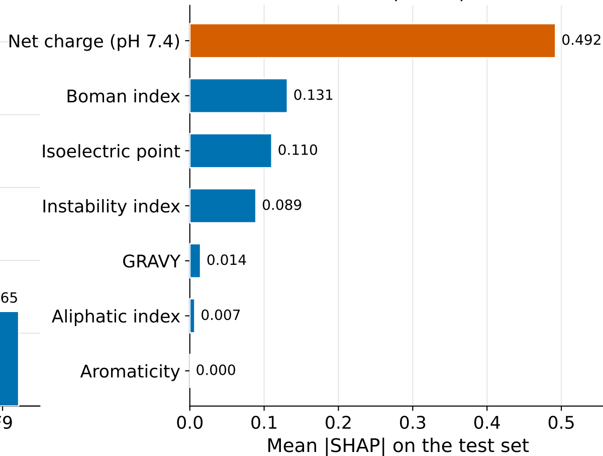
XGBoost descriptor importance
