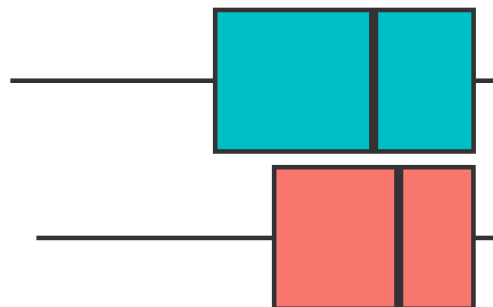
Alphagenome
