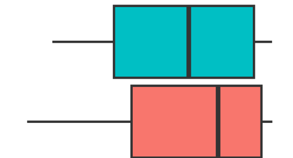
Enformer
