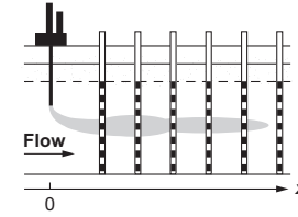
Figure 1.7 The contaminant plume source history reconstruction problem.
