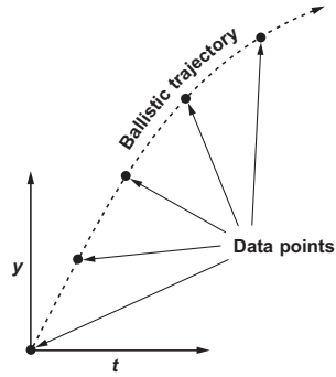
Figure 1.1 The parabolic trajectory problem.
