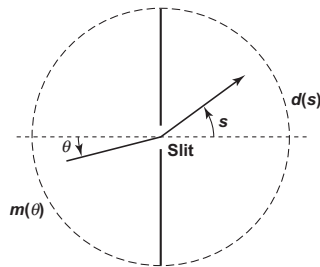
Figure 1.6 The Shaw diffraction intensity problem (1.26).
