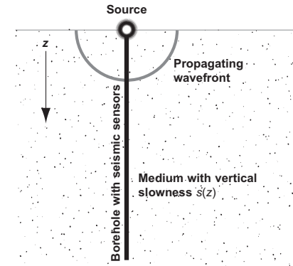
Figure 1.3 The vertical seismic profiling problem.
