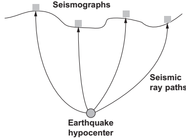
Figure 1.2 The earthquake location problem.
