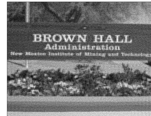
Figure 6.12 CGLS solution, explicit regularization, \alpha = 7.0 \times 10^{-4} .
