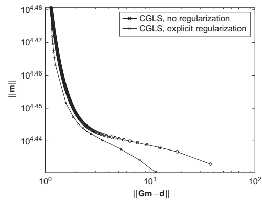
Figure 6.9 L-curves for CGLS deblurring.
