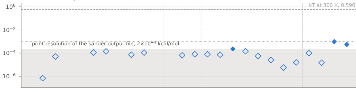
(b) sander – OpenMM n = 20, median 7.6 \times 10^{-5} kcal/mol
