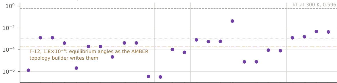
(a) MOSAICS – OpenMM n = 26, median 3.0 \times 10^{-4} kcal/mol
