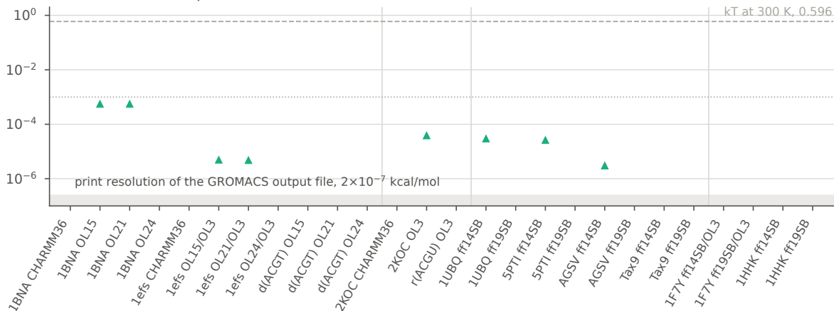
(c) GROMACS – OpenMM n = 8, median 2.9 \times 10^{-5} kcal/mol
