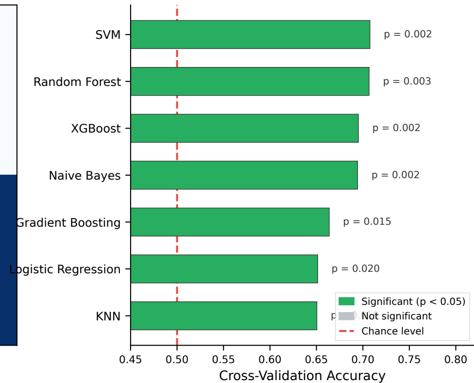
c Permutation Test Results
