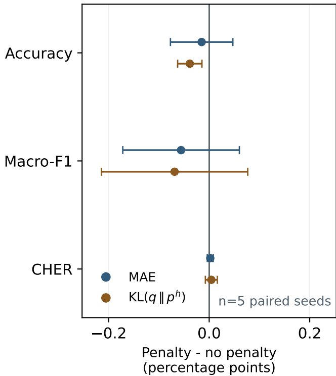
NPD-Rice-COCO-43
