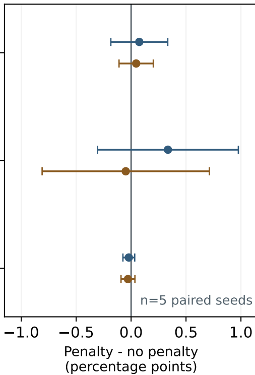
MultiCrop-88
