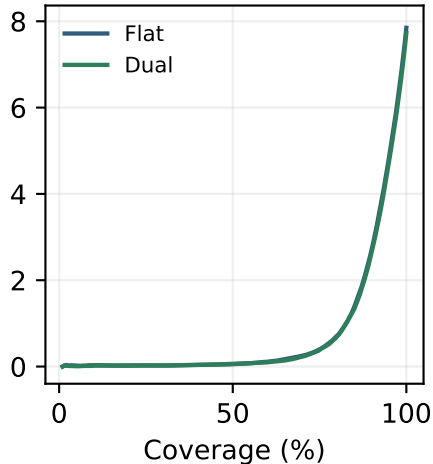
Agri-Foundation-145k
