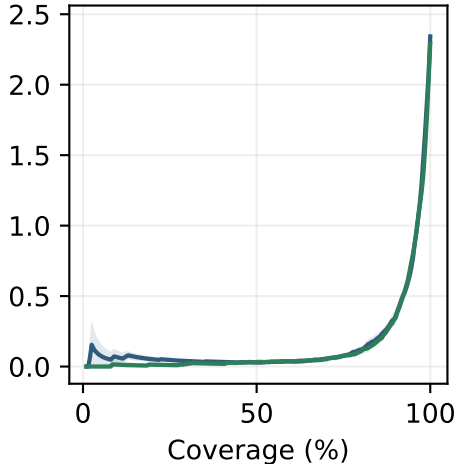
MultiCrop-88
