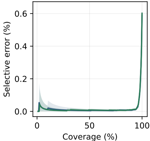
NPD-Rice-COCO-43
