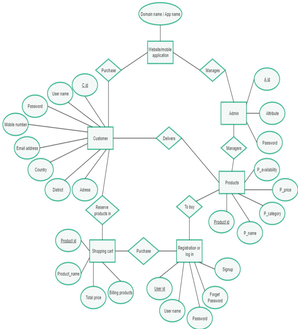
Online Shopping ER Diagram
