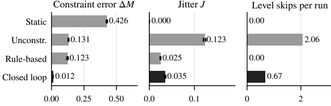
Fig. 3. Main comparison on the test cohort (means, 95% CIs); closed loop dark.
