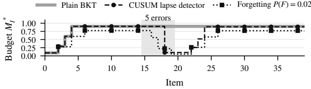
Fig. 4. Scripted probe: 15 correct responses, five errors, then correct again. With plain BKT the estimate is saturated and the budget never moves.
