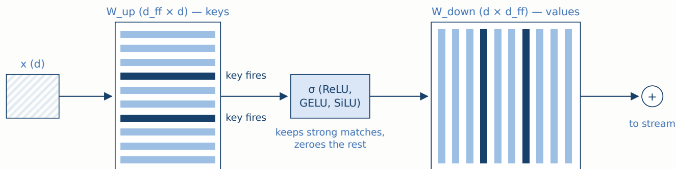
Figure 3.5 — The MLP as a key-value memory. Each row of W_{up} is a key matched against the token's current state; the nonlinearity keeps only the strong matches (dark rows); the corresponding columns of W_{down} (dark columns) are the values added to the residual stream. Two keys fired here, so two values were written.
