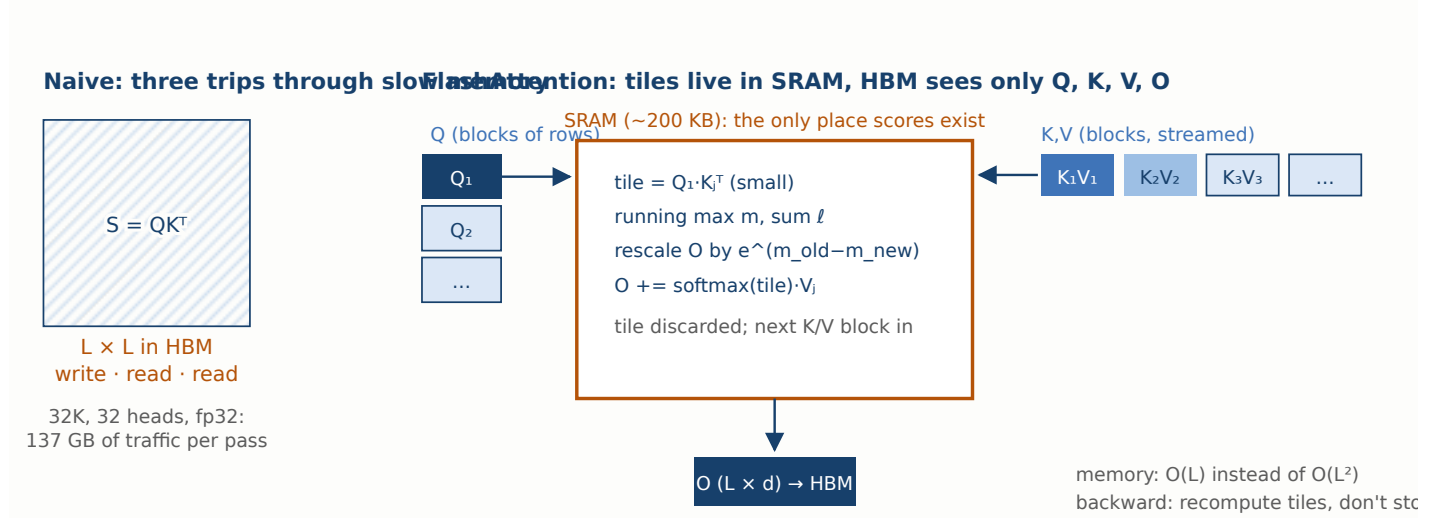
Figure 13.2 — The tiling idea. A block of queries is pinned in fast on-chip memory while key/value blocks stream past it; each score tile is computed, folded into the running output with the online-softmax rescaling, and discarded. The full score matrix never exists anywhere. The result is exact — this is an IO optimization , not an approximation. Watch it move: the attention hub 's FlashAttention tab animates these tiles streaming between HBM and SRAM, with a live counter of the memory round trips a naive kernel would be making.
