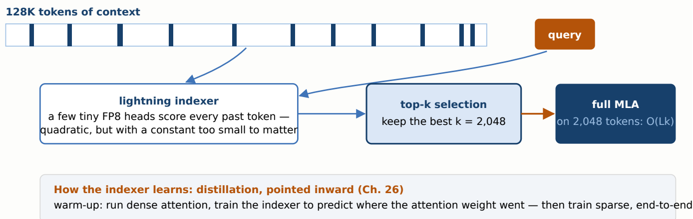
Figure 13.7 — DeepSeek Sparse Attention (V3.2). A near-free scorer chooses 2,048 tokens; the expensive attention runs only there. Note the compounding with §13.3: MLA shrank what each token costs to cache, DSA shrinks how many cached tokens each new token must read . 23
