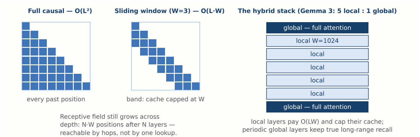
Figure 13.5 — Restricting who sees whom. Left: the causal triangle becomes a band; compute and cache both stop growing with context. Right: production systems rarely go all-local — they interleave windowed layers with full-attention layers, tuning the ratio (Gemma 2 used 1:1 at W=4096 ; Gemma 3, 5:1 at W=1024 ) to keep retrieval alive while most layers run cheap. 1213
