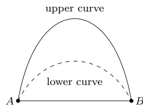
FIGURE 3. Archimedes' convexity postulate.
