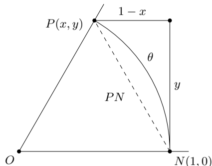
FIGURE 4. Elbow Bounds.
