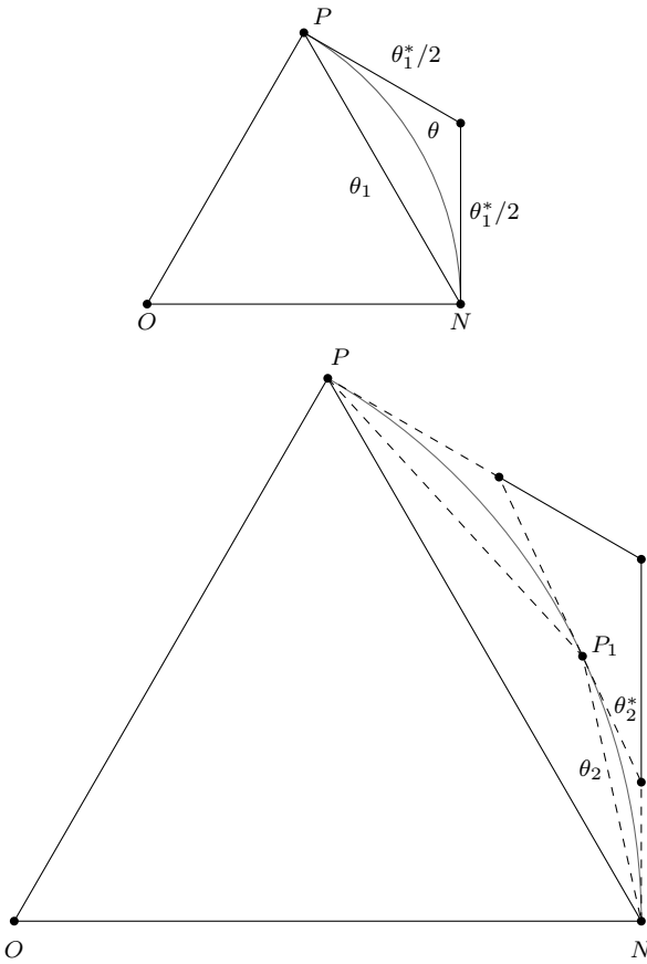
FIGURE 5. Inscribed and circumscribed chords; lower diagram enlarged.
