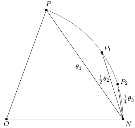
FIGURE 6. Bisection.
