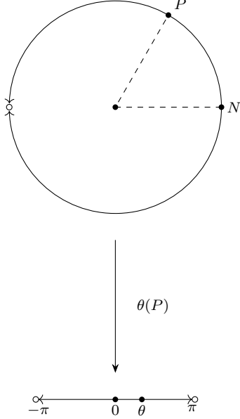
FIGURE 8. Angle measure.
