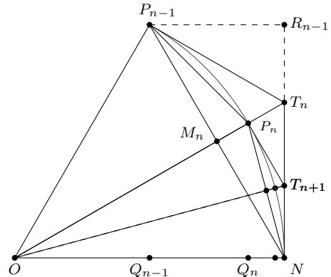
FIGURE 7. First Cut.
