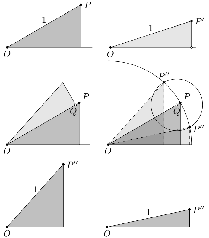
FIGURE 2. Angle stacking.
