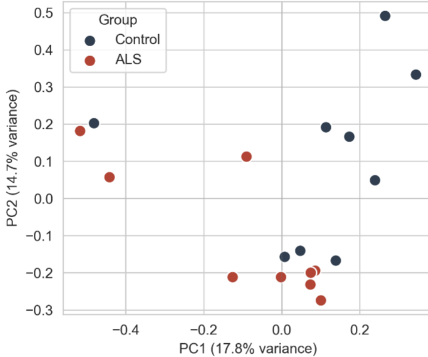
Figure 4: Principal Coordinates Analysis of the Bray-Curtis distances. Each point is one sample, colored red for ALS and blue for Control. The first two principal coordinates explain the variance fraction shown on the axis labels. The two groups overlap visually, but PERMANOVA on the full distance matrix detected significant separation (pseudo- F = 1.7 , p \approx 0.02 ).
