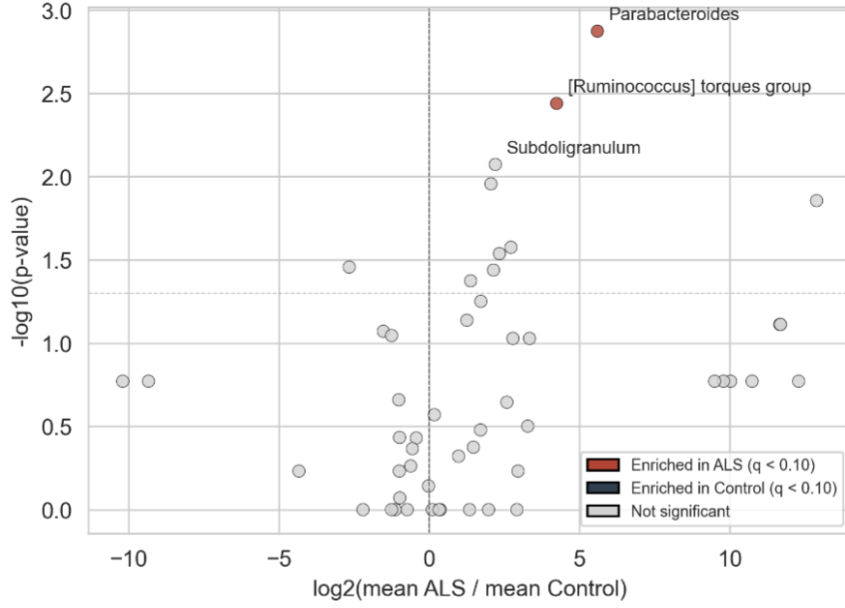
Figure 5: Volcano plot of the per-genus Mann-Whitney U tests. Each point is one genus. The x-axis is the \log_2 ratio of mean relative abundance in ALS over Control, and the y-axis is the -\log_{10} of the raw p-value. Genera passing the FDR threshold of q < 0.10 are colored by direction of change (red for ALS-enriched, blue for Control-enriched); non-significant genera are grey. The horizontal dashed line marks the nominal p = 0.05 . The three genera with the smallest adjusted p-values are labeled.
