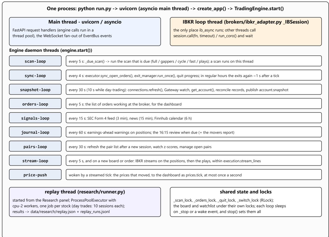
Figure 3 - Threads: everything runs in one Python process; the engine's loops are daemon threads, the replay uses worker processes.
