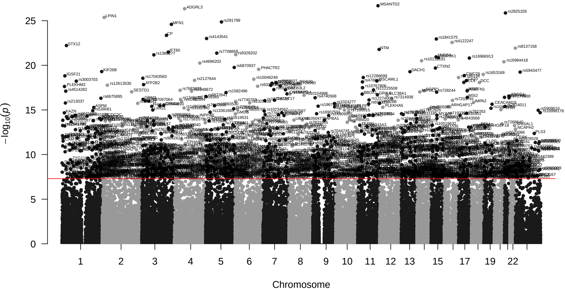
Manhattan Plot: PC1 Association
