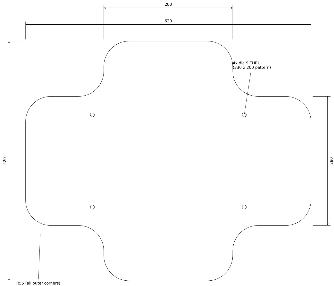
BASE PLATE - TOP VIEW
