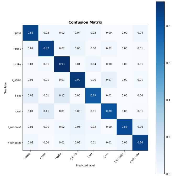
Figure 6. Baseline 8 test confusion matrix. Team-split pooling eliminates the left/right leakage: winpoint recovers to 0.83/0.86 on the diagonal (from B7’s ~0.38), and pass/spike/set no longer swap sides. Remaining errors are within-side (e.g. set vs. spike).
