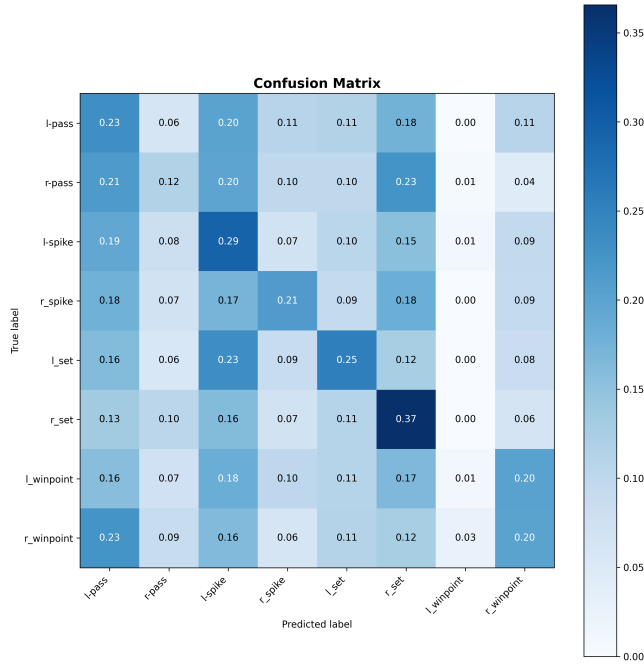
Figure 4. Confusion matrix for Baseline 1 on the test split.
