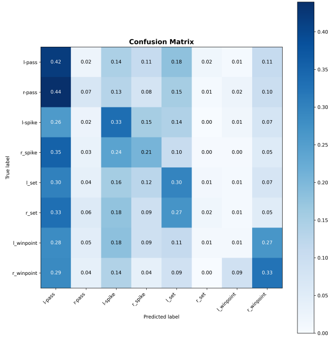
Figure 5. Confusion matrix for Baseline 3 (run2 checkpoint) on the test split.
