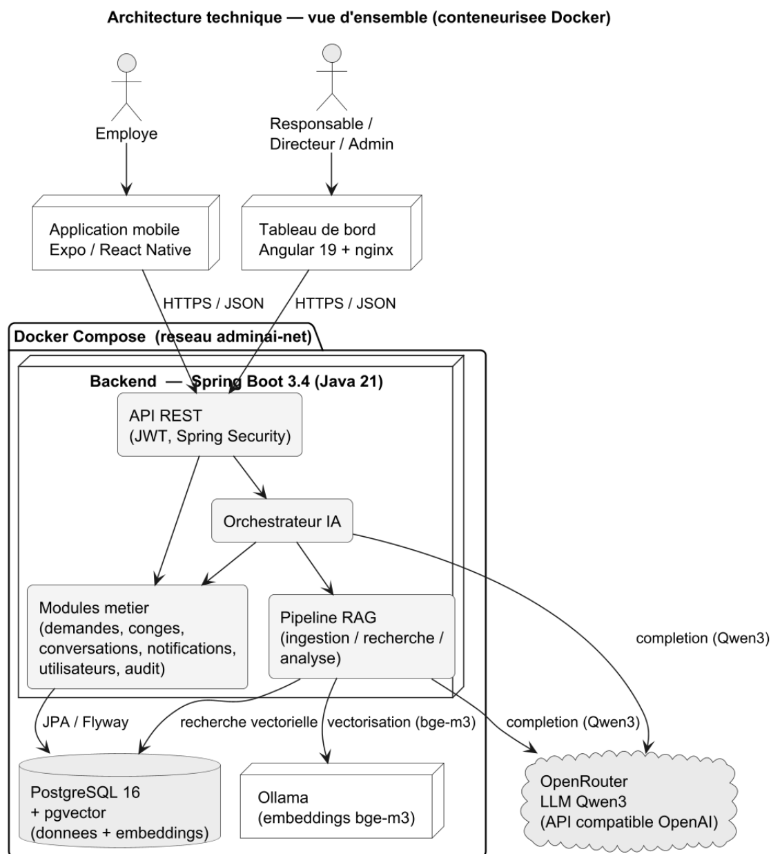
Figure 3.1. Architecture technique conteneurisée
