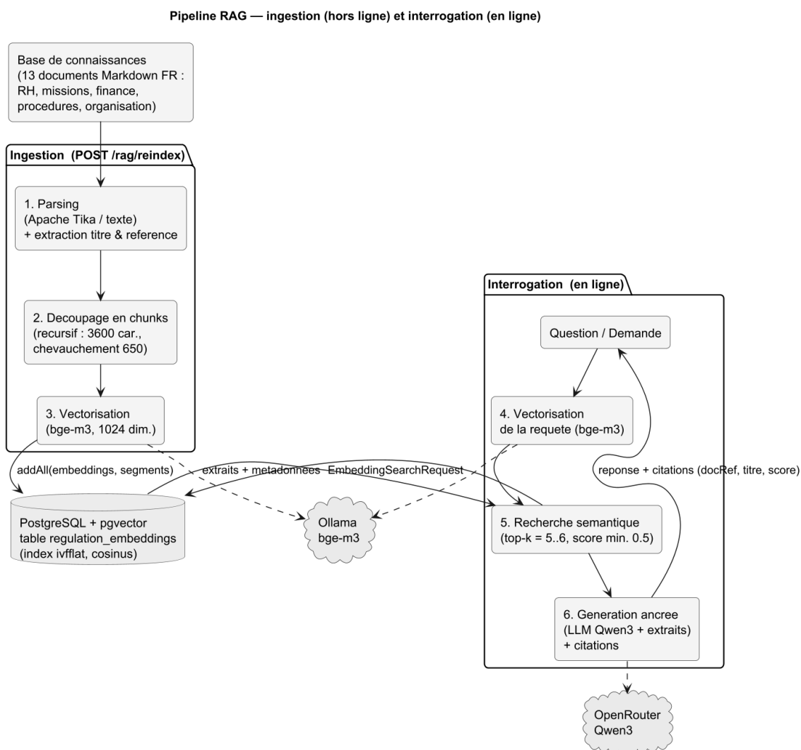
Figure 4.1. Pipeline RAG : ingestion et interrogation
