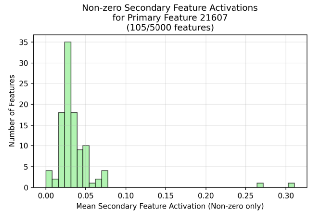
Figure 2. Distribution of secondary features (features from secondary SAE trained on NFM embedding) mean activation values when only primary feature (21607, Emotion) is naturally activated by our stimulus set. Only non-zero features are shown (vast majority are zero). Note: The other primary feature (21781, Formality, not shown here ) produces a very similar secondary feature activation distribution.
