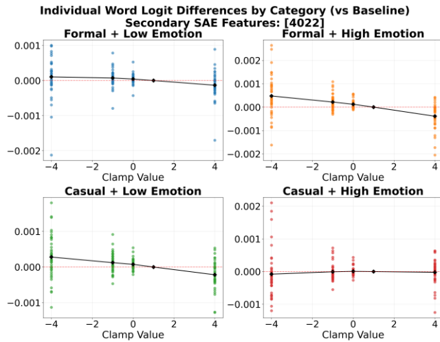
Figure 3. X-axis : Clamping values ( -4 , -1 , 0 , 1 , 4 ) of integration feature, #4022. Y-axis : Reconstructed logit differences from baseline. Four graphs : 2 \times 2 category of high/low for selected features (Emotion, Formality). Note the differential impact of the integration feature on bottom right (low Formality, high Emotion; reverse direction) driving the statistically significant ANOVA interaction, showcasing how the two features nonlinearly combine.
