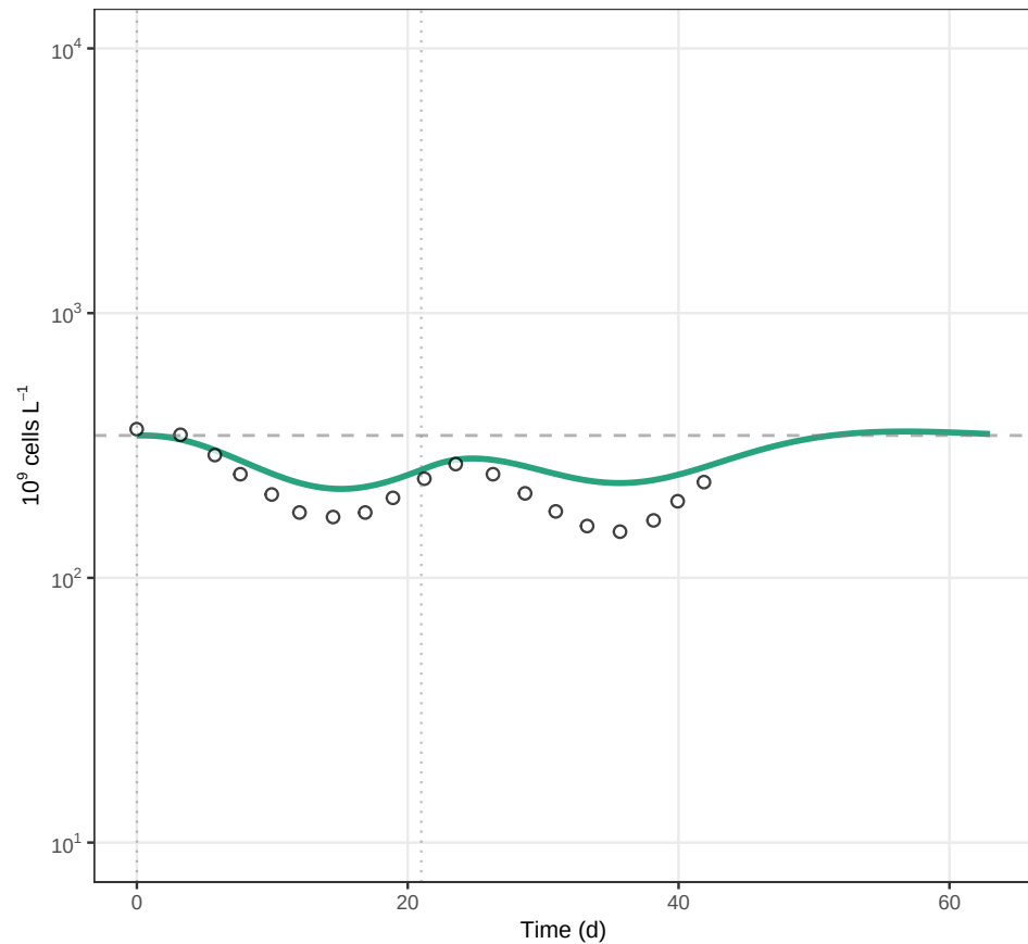
Platelets
