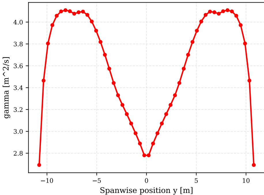
Leading Edge Total Circulation Distribution (VLM)
