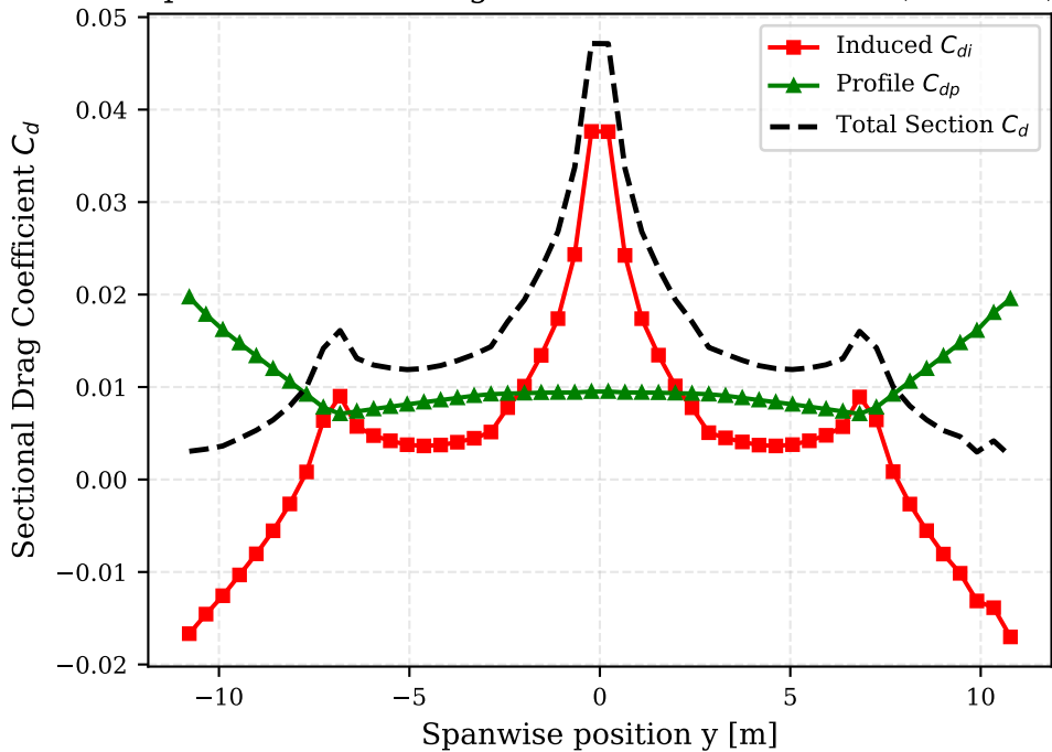
Spanwise Local Drag Coefficient Distribution (NL-VLM)
