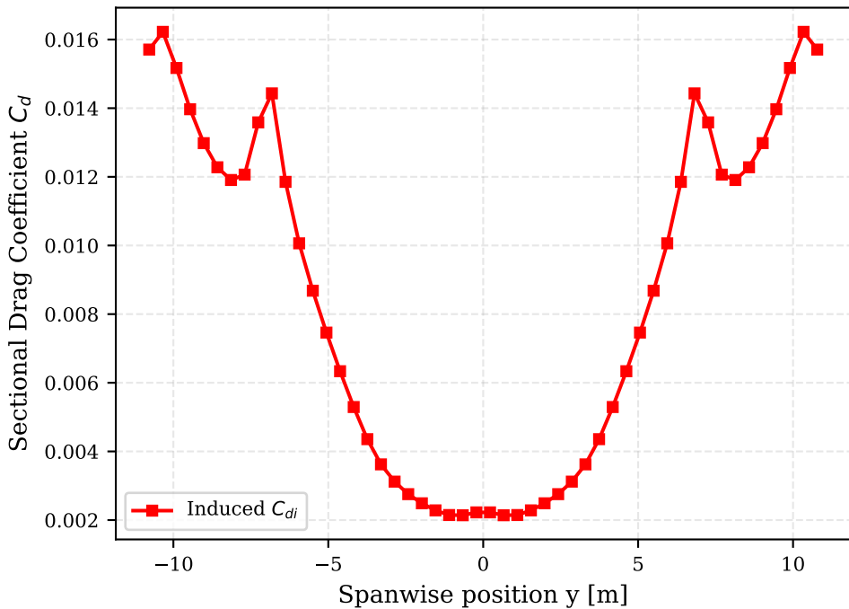
Spanwise Local Drag Coefficient Distribution (VLM)
