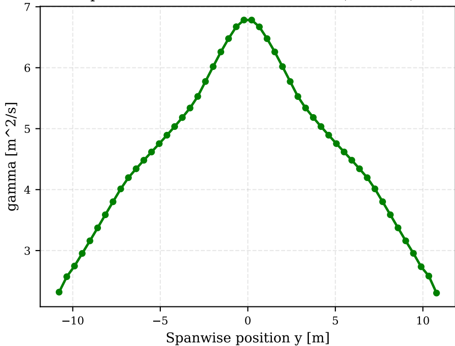
Spanwise Circulation Distribution (NL-VLM)
