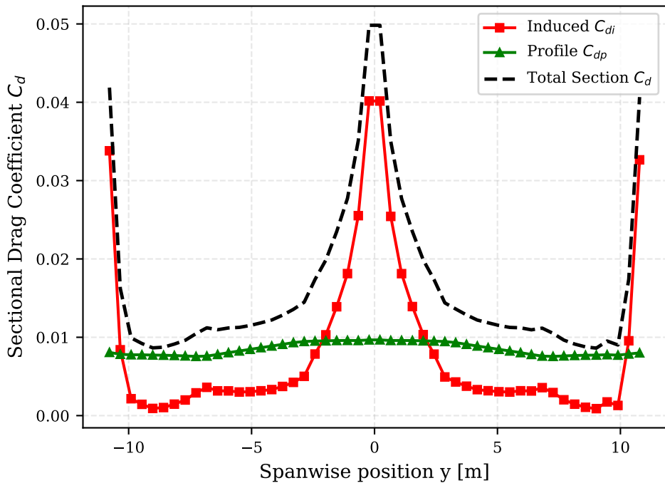
Spanwise Local Drag Coefficient Distribution (NL-VLM)
