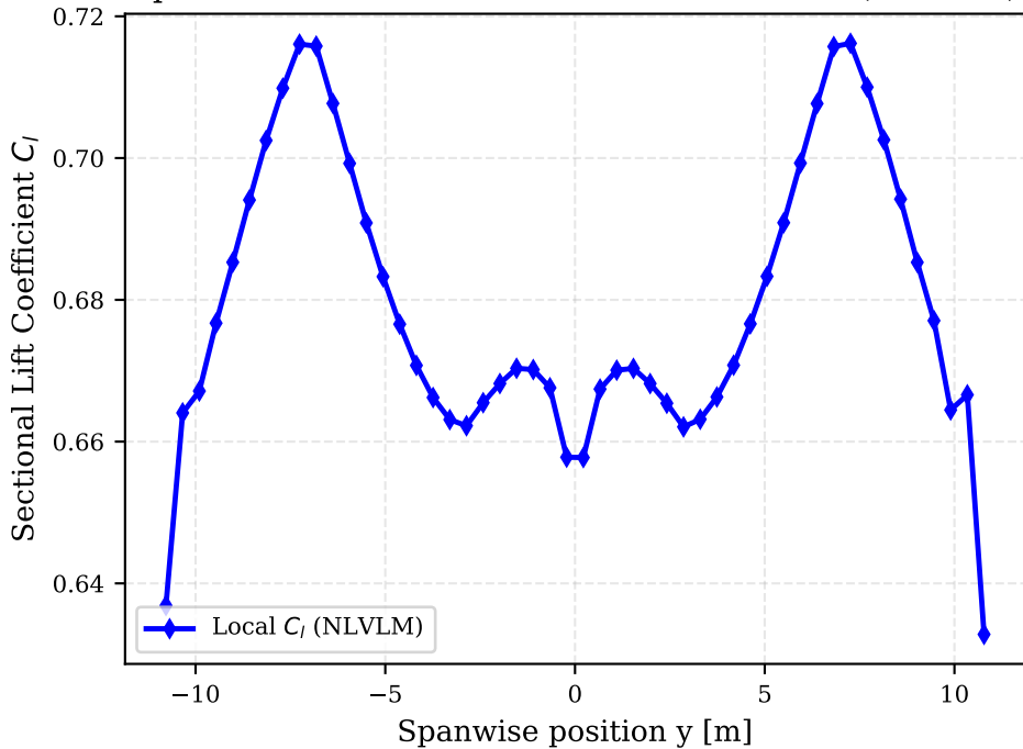
Spanwise Local Lift Coefficient Distribution (NL-VLM)
