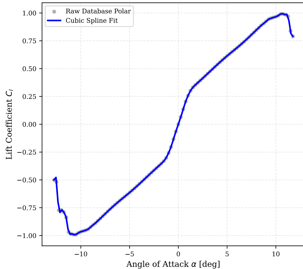
Lift Coefficient C_l vs \alpha (N0012 @ Re=100,000)
