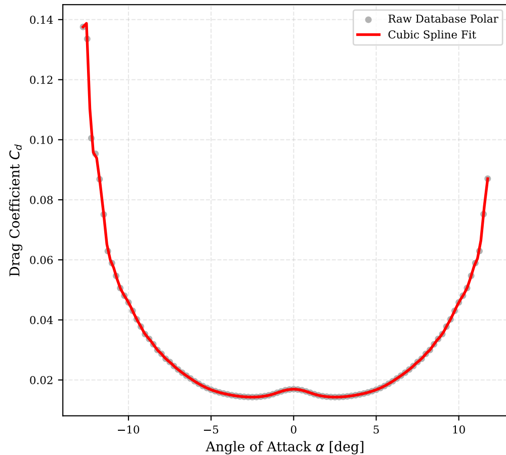
Drag Coefficient C_d vs \alpha (N0012 @ Re=100,000)
