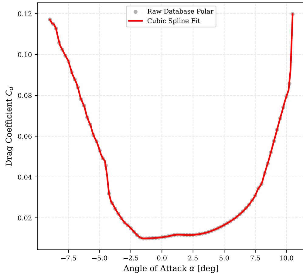
Drag Coefficient C_d vs \alpha (AG18 @ Re=100,000)
