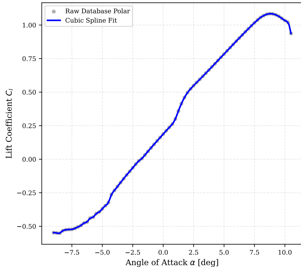
Lift Coefficient C_l vs \alpha (AG18 @ Re=100,000)
