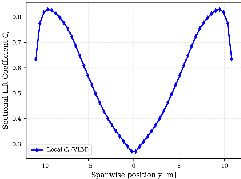
Spanwise Local Lift Coefficient Distribution (VLM)
