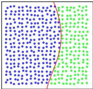
Final Clustering
