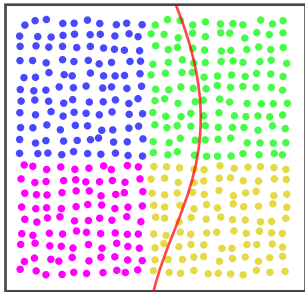
Initial Clustering
