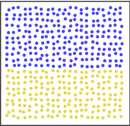
Un-mixed Clusters
