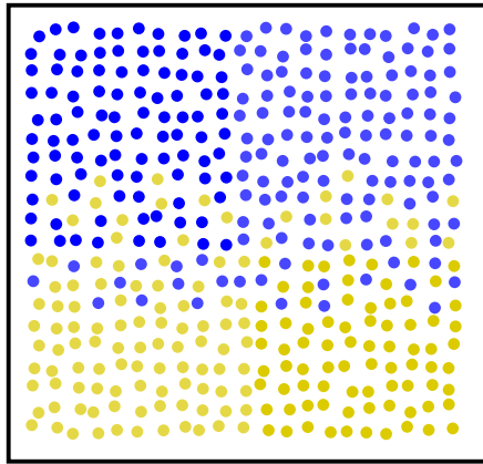
Mixed Clusters
